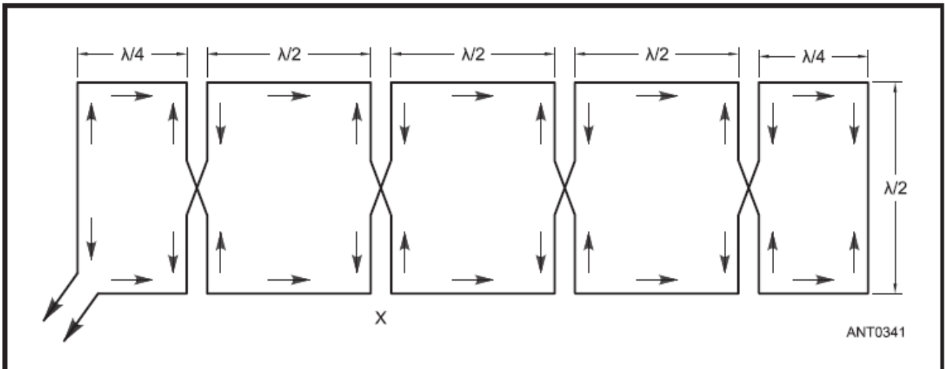
Figure 12.13 — Typical Sterba array, an 8-element version.
